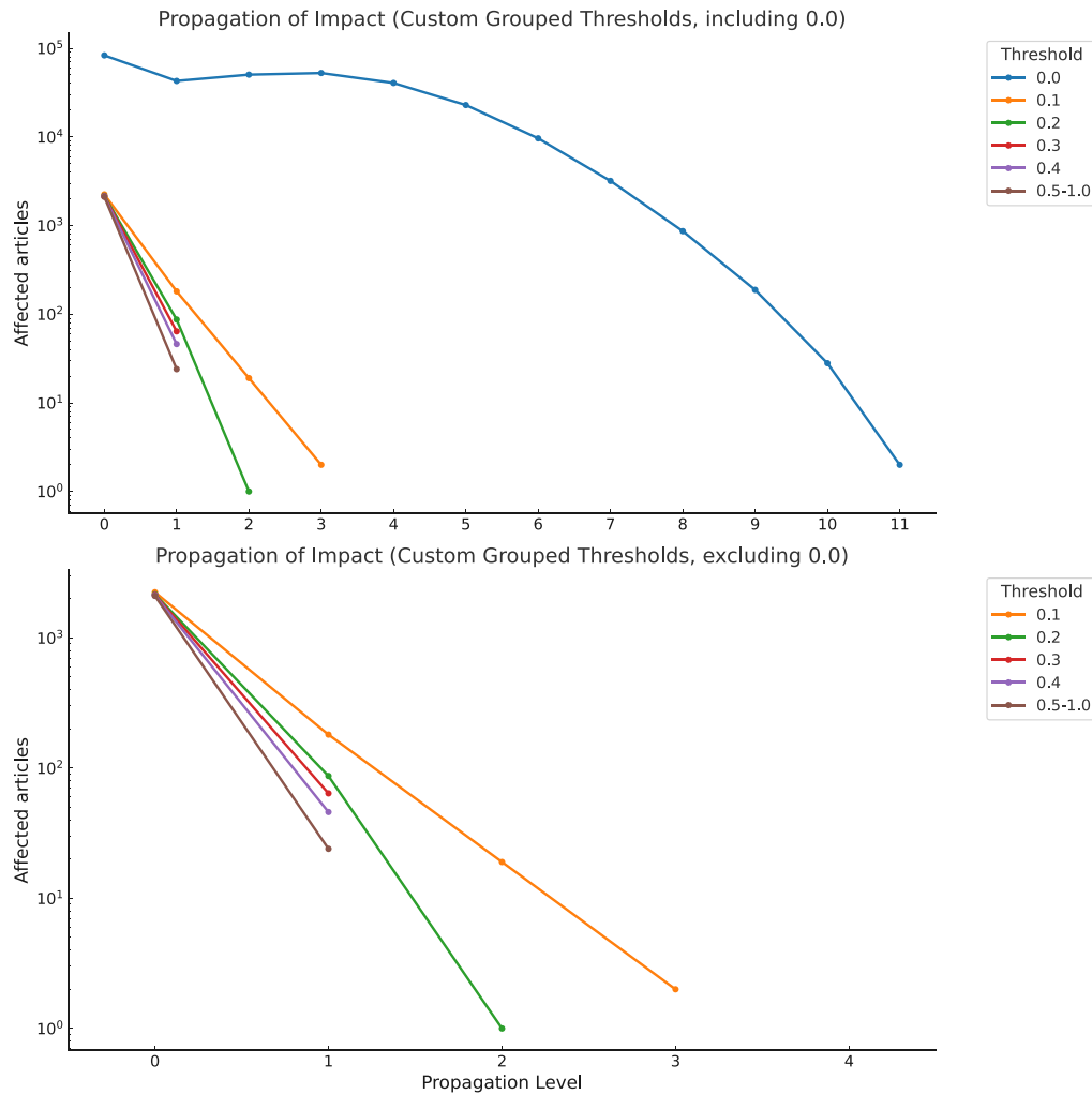
Fig. 9. Propagation impact under the Affection-Transmission model for different threshold values. The upper panel includes the degenerate case \iota = 0.0 , corresponding to unrestricted propagation, while the lower panel excludes this case to highlight differences among positive thresholds. Threshold values are treated as a structural control parameter rather than as empirically calibrated quantities. Results show that \iota = 0.0 defines a worst-case regime with unbounded propagation, whereas all \iota > 0 lead to rapidly constrained propagation, indicating robustness of the qualitative behaviour across positive threshold values.
