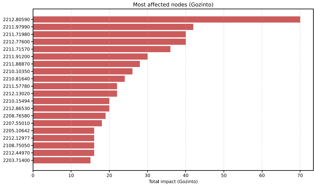
Fig. H.1. Nodes receiving the highest cumulative impact according to the Gozinto model. Bars represent the total impact received from affected citation paths, highlighting articles that are structurally most exposed to upstream dataset unavailability. Comparison with propagated-impact rankings shows that highly affected nodes do not necessarily act as superpropagators, underscoring the presence of distinct structural roles within the citation network.
